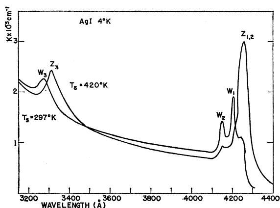
FIG. 1. Exciton spectrum of AgI at 4°K.
