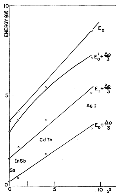
FIG. 4. Main peaks in the absorption spectrum of the AgI isoelectronic sequence (corrected for spin-orbit splitting.)
