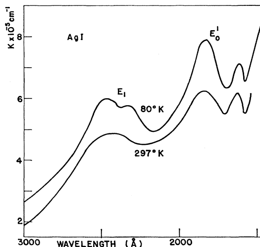
FIG. 8. High-energy absorption spectrum of AgI.
