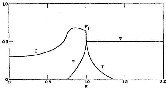
FIG. 15. Density of states and polarizability around an S_2 -type saddle point.
